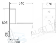
LJ-305 Two piece toilet Size: 640x370x805 mm S-trap: 100-250 mm roughing-in P-trap: 180 mm roughing-in
