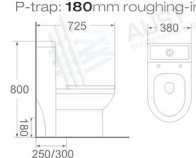
LJ-102 One piece toilet Size: 725x380x800 mm S-trap: 250/300 mm roughing-in P-trap: 180 mm roughing-in
