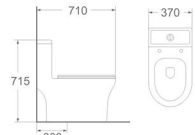
LJ-108 One piece toilet Size: 710x370x715 mm S-trap: 300 mm roughing-in
