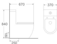
LJ-103 One piece toilet Size: 670x370x840 mm S-trap: 250 mm roughing-in P-trap: 180 mm roughing-in
