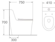
LJ-118 One piece toilet Size: 750x410x700 mm S-trap: 300 mm roughing-in
