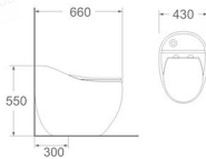
LJ-121 One piece toilet Size: 660x430x550 mm S-trap: 300 mm roughing-in
