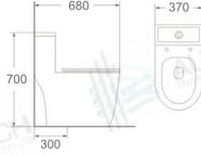
LJ-113 One piece toilet Size: 680x370x700 mm S-trap: 300 mm roughing-in
