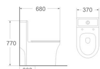
LJ-109 One piece toilet Size: 680x370x770 mm S-trap: 300 mm roughing-in
