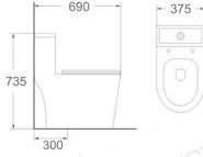
LJ-112 One piece toilet Size: 690x375x735 mm S-trap: 300 mm roughing-in
