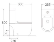
LJ-316 Two piece toilet Size: 660x365x800 mm S-trap: 250 mm roughing-in P-trap: 180 mm roughing-in
