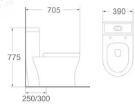
LJ-104 One piece toilet Size: 705x390x775 mm S-trap: 250/300 mm roughing-in
