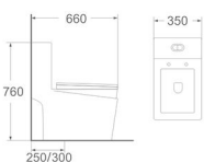
LJ-124 One piece toilet Size: 660x350x760 mm S-trap: 250/300 mm roughing-in
