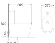
LJ-320 Two piece toilet Size: 605x370x800 mm S-trap: 100-250 mm roughing-in P-trap: 180 mm roughing-in
