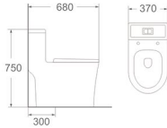
LJ-115 One piece toilet Size: 680x370x750 mm S-trap: 300 mm roughing-in
