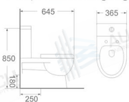
LJ-311 Two piece toilet Size: 645x365x850 mm S-trap: 250 mm roughing-in P-trap: 180 mm roughing-in
