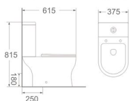
LJ-308 Two piece toilet Size: 615x375x815 mm S-trap: 250 mm roughing-in P-trap: 180 mm roughing-in
