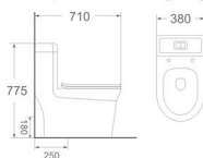
LJ-127 One piece toilet Size: 710x380x775 mm S-trap: 250 mm roughing-in P-trap: 180 mm roughing-in
