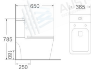
LJ-306 Two piece toilet Size: 650x365x785 mm S-trap: 250 mm roughing-in P-trap: 180 mm roughing-in
