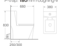
LJ-106 One piece toilet Size: 680x380x830 mm S-trap: 250/300 mm roughing-in P-trap: 180 mm roughing-in
