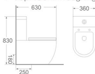
LJ-303 Two piece toilet Size: 630x360x830 mm S-trap: 250 mm roughing-in P-trap: 180 mm roughing-in
