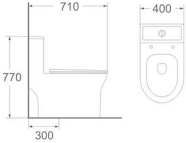
LJ-110 One piece toilet Size: 710x400x770 mm S-trap: 300 mm roughing-in
