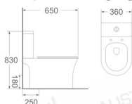
LJ-310 Two piece toilet Size: 650x360x830 mm S-trap: 250 mm roughing-in P-trap: 180 mm roughing-in
