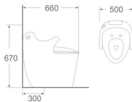
LJ-123 One piece toilet Size: 660x500x670 mm S-trap: 300 mm roughing-in
