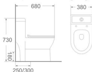
LJ-125 One piece toilet Size: 680x380x730 mm S-trap: 250/300 mm roughing-in P-trap: 180 mm roughing-in
