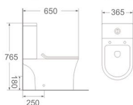
LJ-309 Two piece toilet Size: 650x365x765 mm S-trap: 250 mm roughing-in P-trap: 180 mm roughing-in
