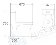
LJ-101 One piece toilet Size: 670x370x750 mm S-trap: 300 mm roughing-in
