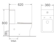
LJ-312 Two piece toilet Size: 620x360x800 mm S-trap: 250 mm roughing-in P-trap: 180 mm roughing-in
