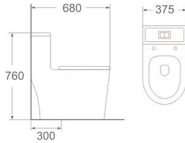
LJ-116 One piece toilet Size: 680x375x760 mm S-trap: 300 mm roughing-in
