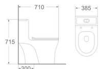
LJ-107 One piece toilet Size: 710x385x715 mm S-trap: 300 mm roughing-in
