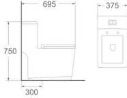
LJ-111 One piece toilet Size: 695x375x750 mm S-trap: 300 mm roughing-in
