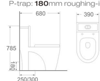
LJ-105 One piece toilet Size: 680x390x785 mm S-trap: 250/300 mm roughing-in P-trap: 180 mm roughing-in
