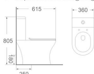
LJ-315 Two piece toilet Size: 615x360x805 mm S-trap: 250 mm roughing-in P-trap: 180 mm roughing-in
