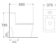
LJ-126 One piece toilet Size: 690x375x785 mm S-trap: 250 mm roughing-in P-trap: 180 mm roughing-in
