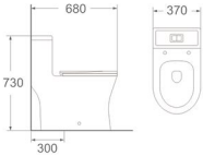
LJ-114 One piece toilet Size: 680x370x730 mm S-trap: 300 mm roughing-in
