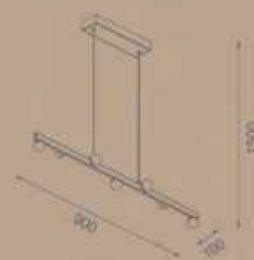
DCD01804 Pendant Lamp Black 900X100XH1500MM LED 3000K 25W Metal+Acrylic
