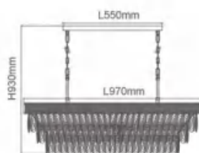
DCD00230 Pendant Lamp Metal+Crystal Brass Gold+Black 970*310*330MM E14*13
