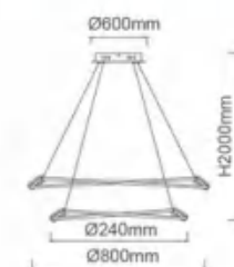
DCD00789 / DCD00790 Pendant Lamp 80W D600+800* H2000mm Brass Gold / Chrome Iron+Crystal
