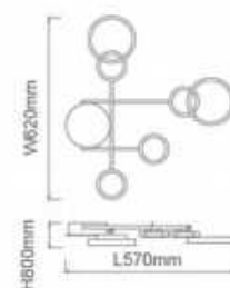
DCB015093 Wall Lamp 620*570mm Brass Gold LED 23W Aluminum + silicon
