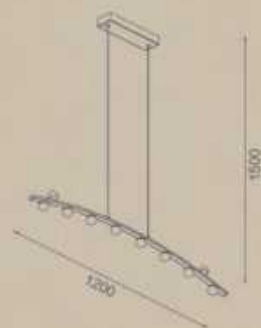
DCD01200 Pendant Lamp Black 1200*100*H1500MM LED 3000K 36W Metal+Acrylic
