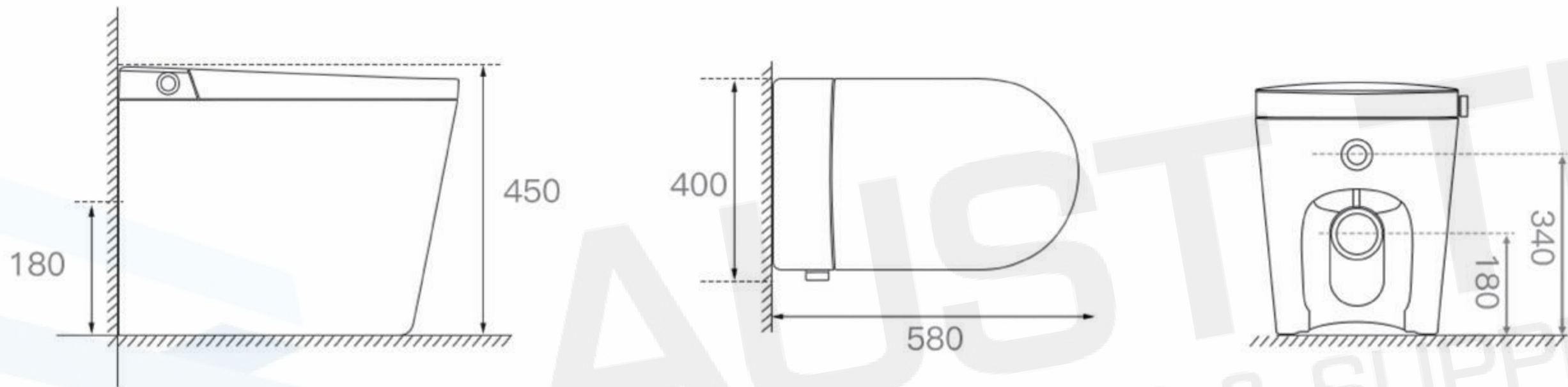
Dimension drawing (size:mm)
