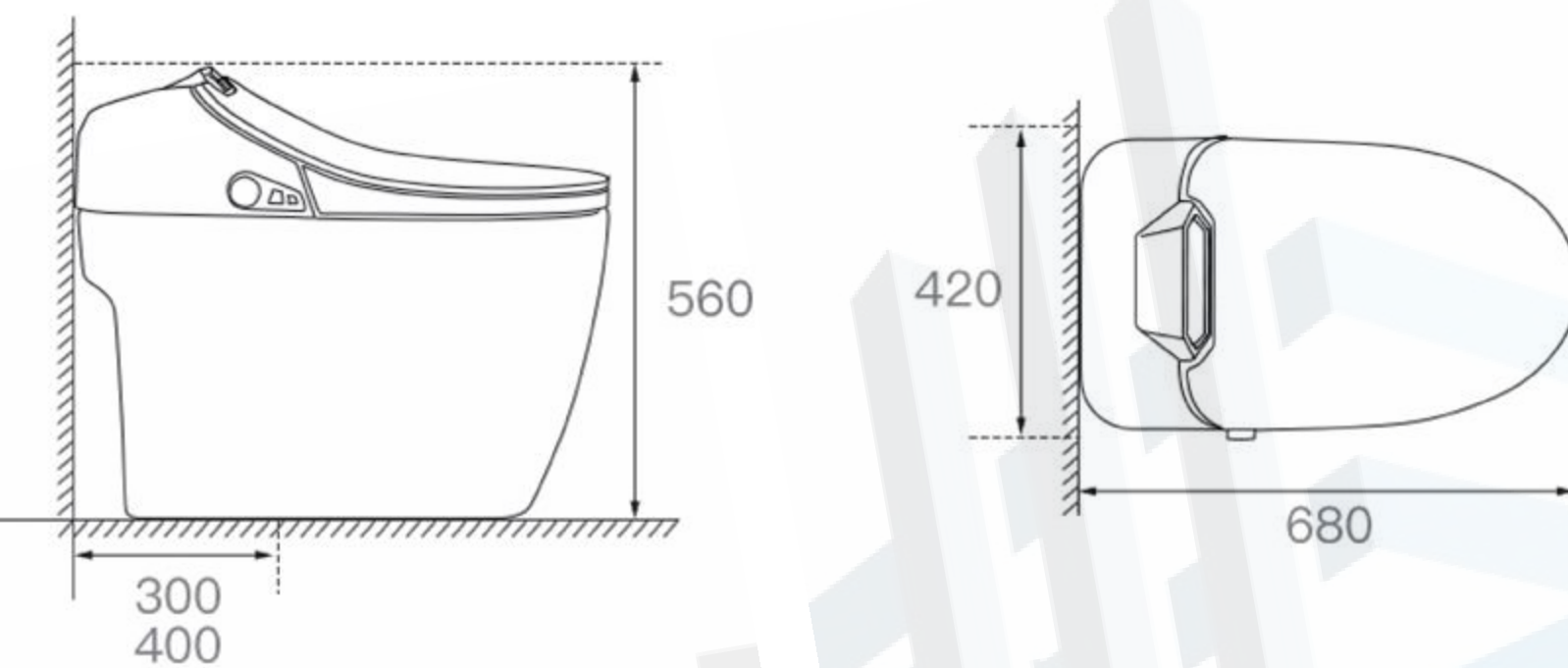
Dimension drawing (size:mm)
