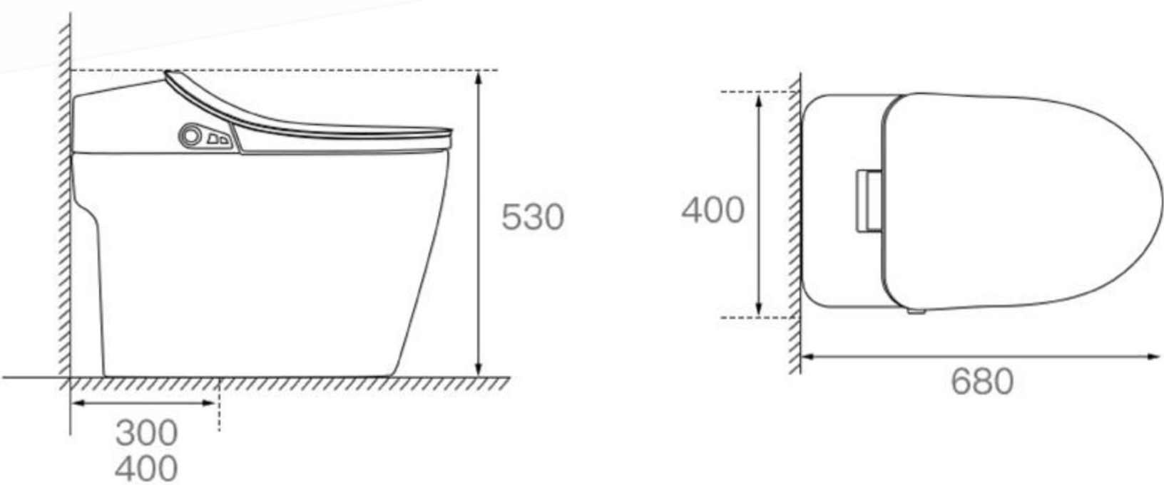
Dimension drawing (size:mm)
