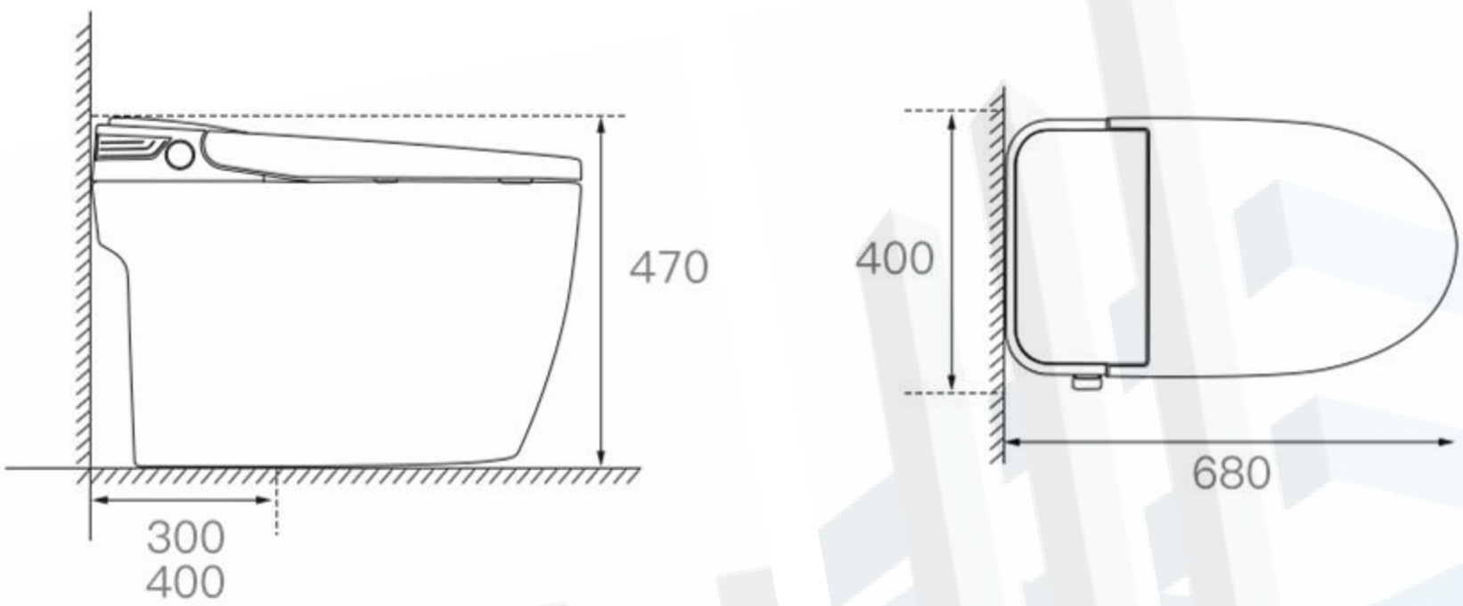
Dimension drawing (size:mm)
