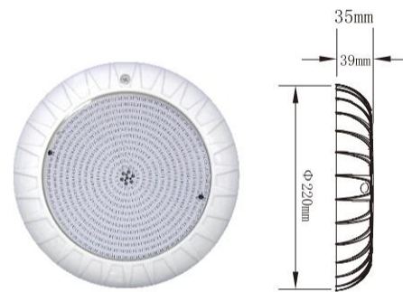
PK8002 Wall mounted type pool light
