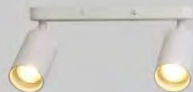
WT233266X-2B Aluminium+Iron 2*GU10 L260*W105*H127 SWH
