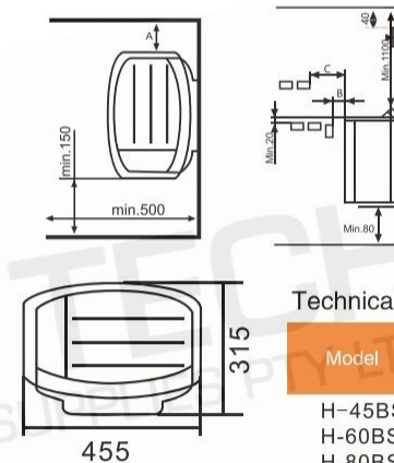
Installation dimension
