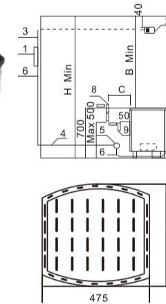
Installation dimension
